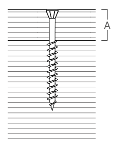
A maximum fastening thickness
