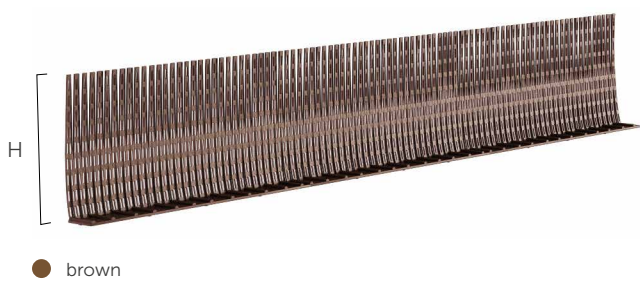
④ BIRD COMB EVO with 25 mm batten and H= 130 mm
